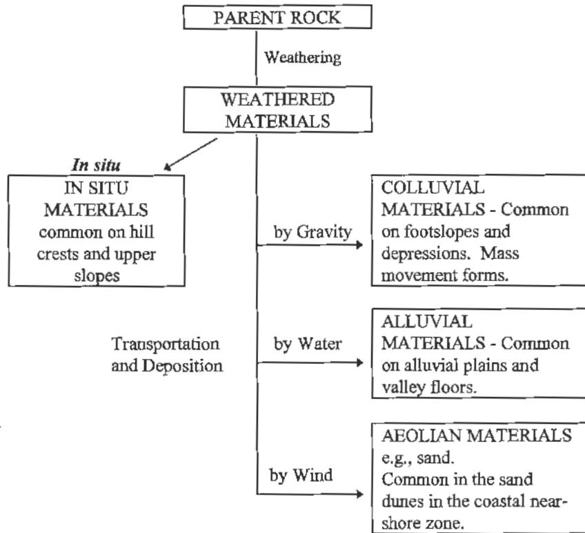
Fig. 8 Origin of parent materials
