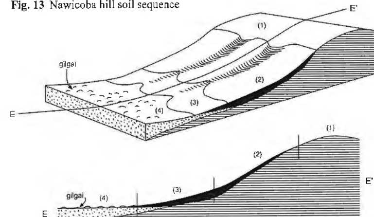
Fig. 13 Nawicoba hill soil sequence
