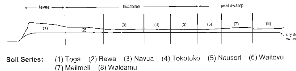
Fig. 11 Rewa delta alluvial sequence
