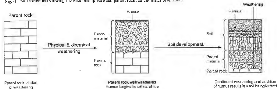
Fig. 4 Soil formation showing the relationship between parent rock, parent material and soil.
