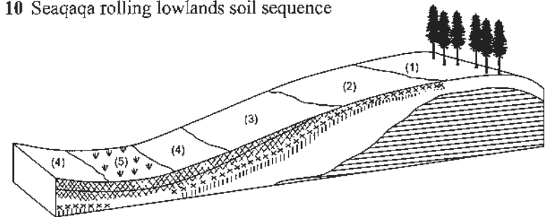
Fig. 10 Seaqaqa rolling lowlands soil sequence
