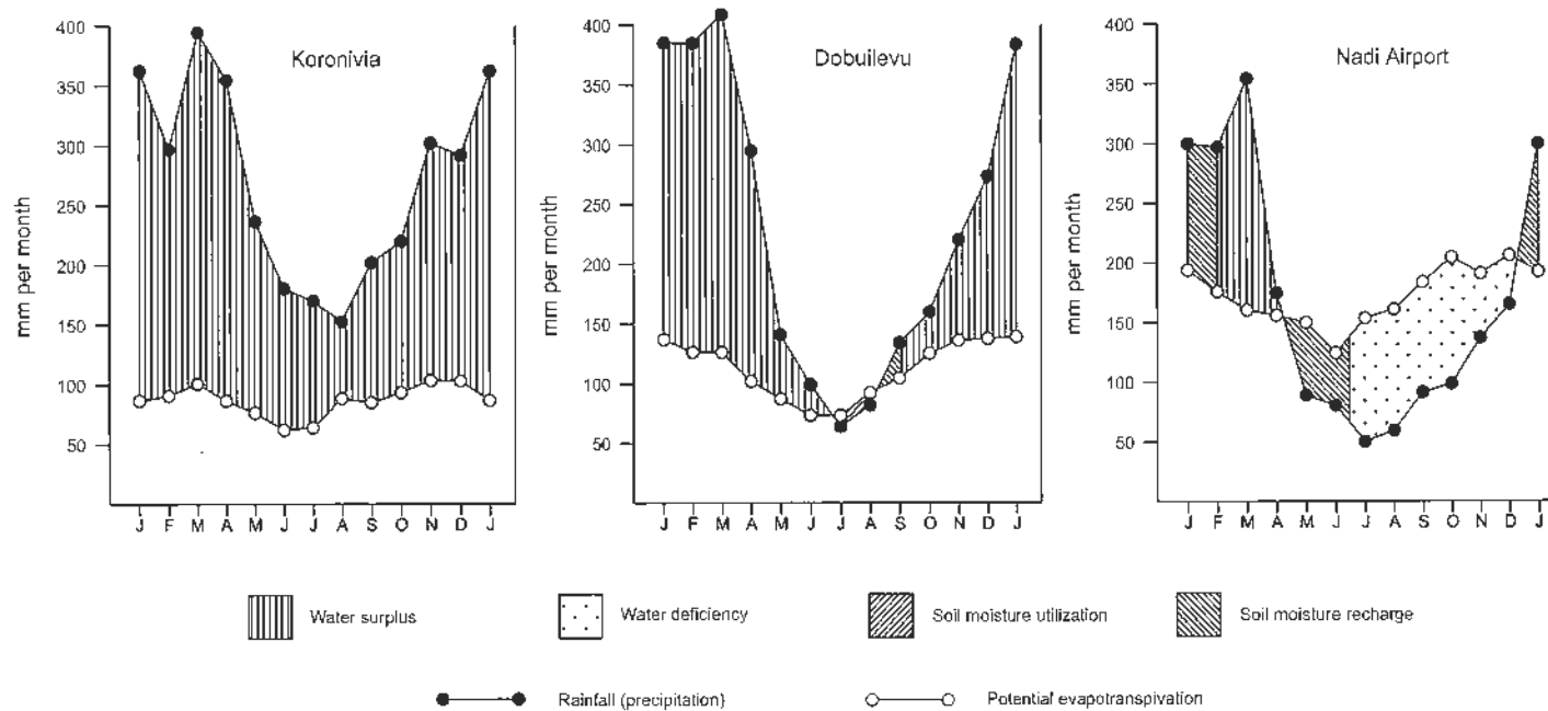
Fig. 16 Soil moisture balances for contrasting areas of Vitu Levu
